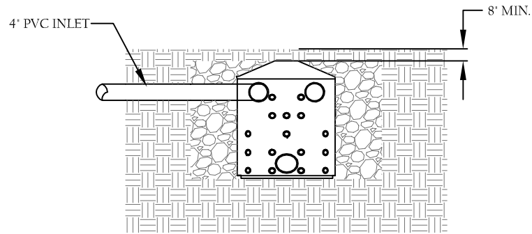
SECTION VIEW
